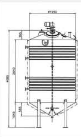
REF CB5272 KALIBER ENG. 8000L, 48BRL, YEAST TANK S/S 316 INSULATED, TWIN JACKETED & AGITATED
