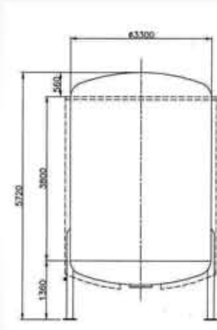
REF CB5260 4X 32,000L, 195BRL, VERTICAL, STAINLESS STEEL, INSULATED VESSELS
