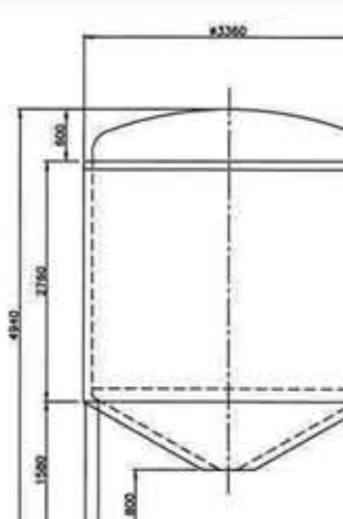
REF CB5273 2X 20,500L, 125BRL, VERTICAL, STAINLESS STEEL, JACKETED, INSULATED & AGITATED VESSELS
