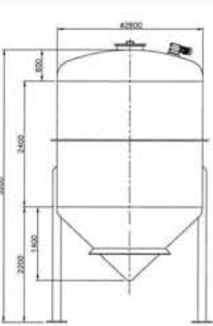
REF CB5270 2X 19,600L, 120BRL, VERTICAL, STAINLESS STEEL & AGITATED VESSELS
