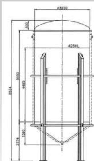
REF CB5251 8X 42,500L, 260BRL, VERTICAL CONICAL BASE INSULATED S/S MATURATION VESSEL WITH LEGS
