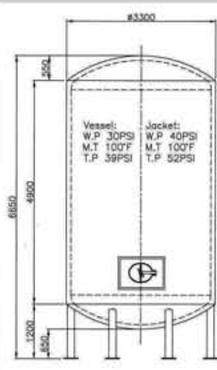
REF CB5249 2X 36,000L, 220BRL, BRIGHT BEER TANKS, S/S, INSULATED & SIDE MOUNTED AGITATOR
