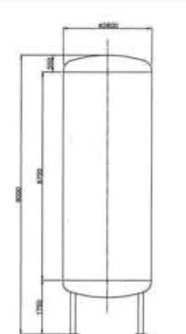
REF CB5245 4X 41,000L, 250BRL, BRIGHT BEER STAINLESS STEEL VESSELS, WP 1.2Bar TP 1.4Bar
