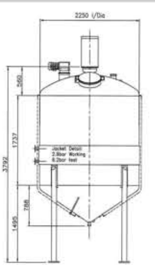
REF CB5264 - 4X 9,000L, 55 BRL, VERTICAL S/S JACKETED & INSULATED AGITATED YEAST VESSELS
