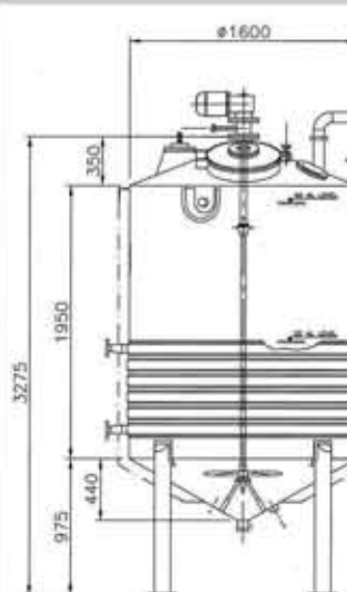
REF CB5268 2X 4,000L, 24BRL, S/S VERTICAL, JACKETED, INSULATED & AGITATED YEAST VESSELS
