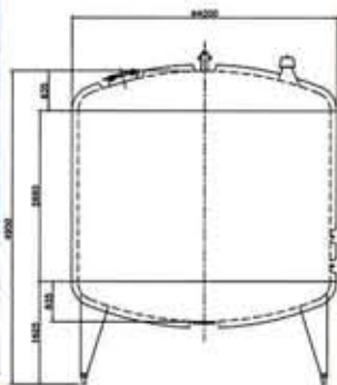
2X 230 BRL, 37,800L STAINLESS STEEL, INSULATED, BRIGHT BEER TANKS
